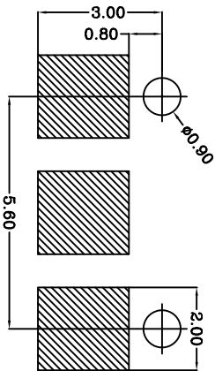
Recommended P.C.B. layout (Component Side)
